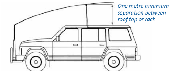
Antenna mounted at bumper bar height
